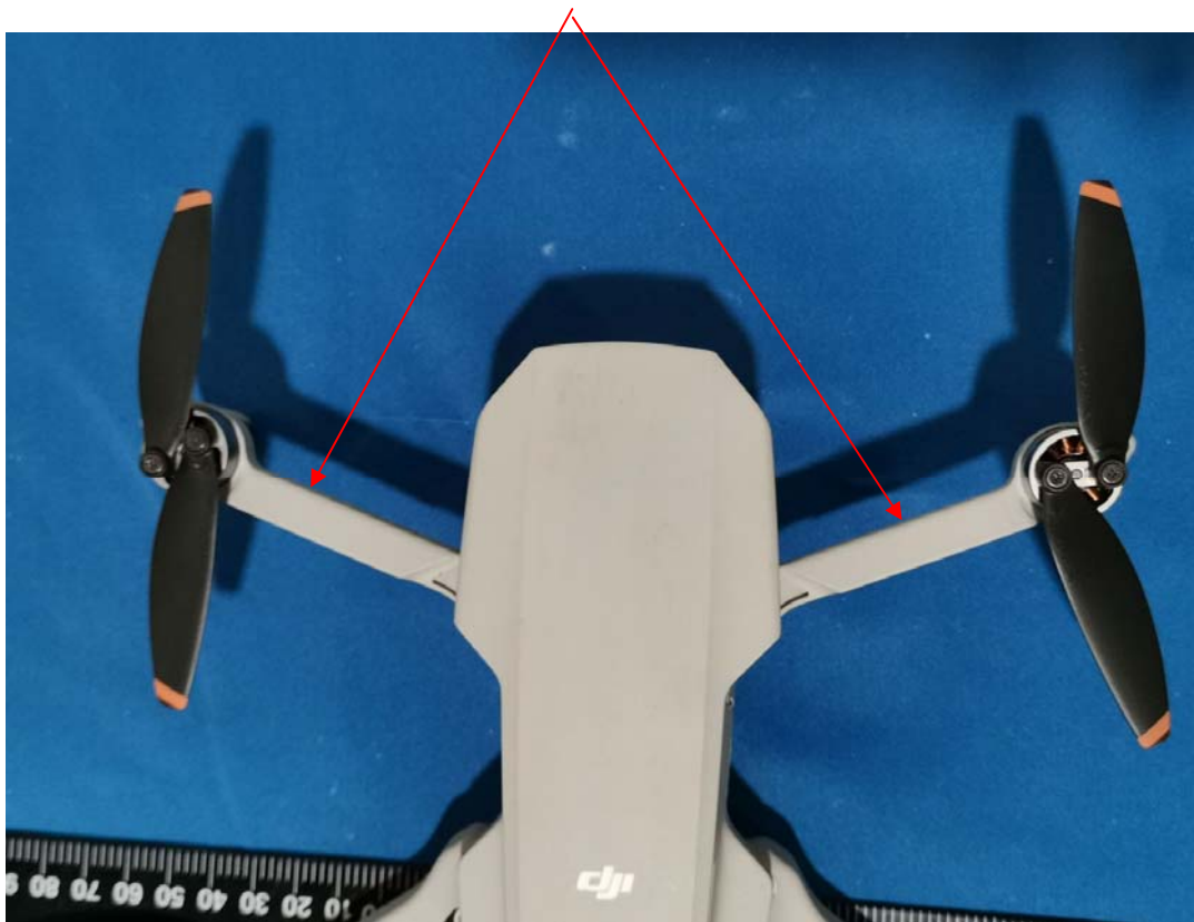
Antenna Location
