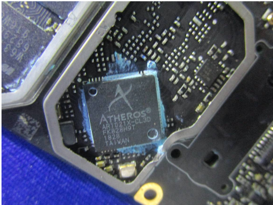
Antenna Chain 0
