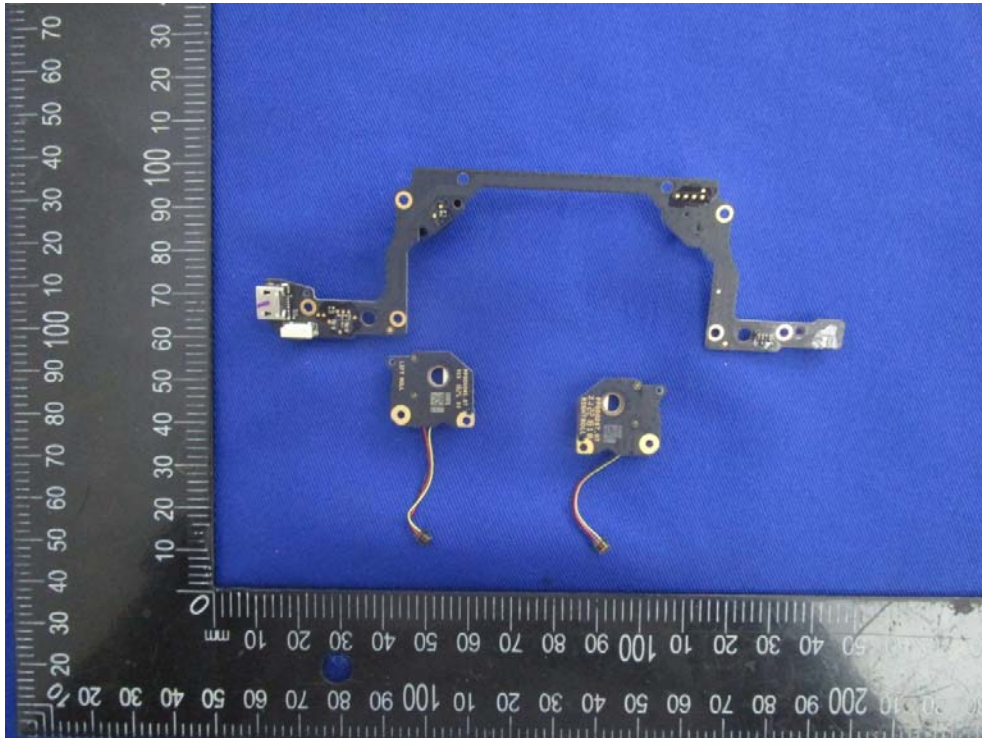
EUT – Button Board Bottom View
