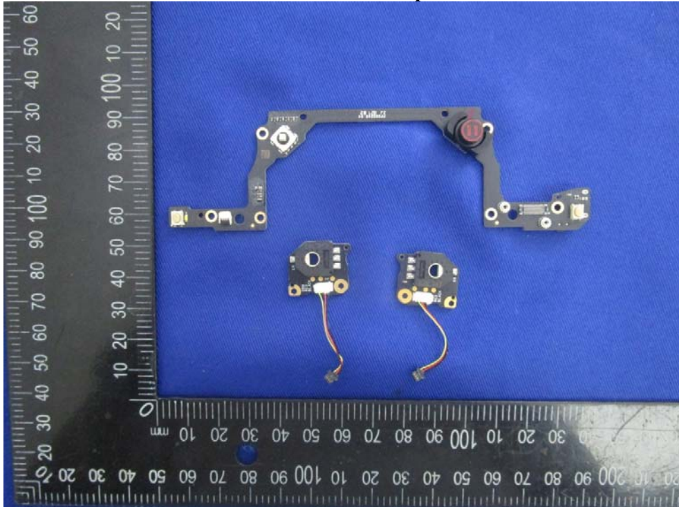
EUT – Button Board Top View
