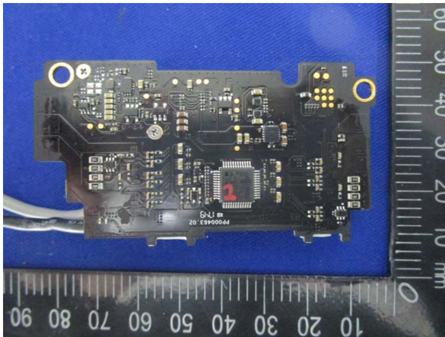
EUT – PCB-12 Bottom View
