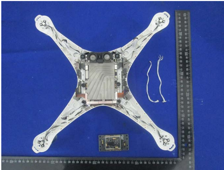
EUT –Uncover-15 View
