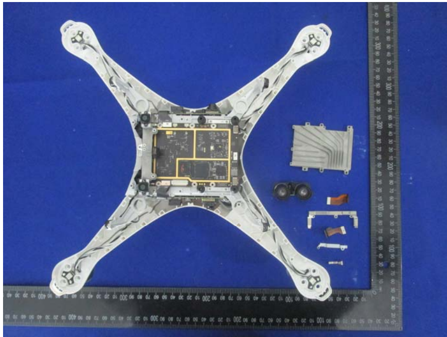
EUT – Uncover-16 View
