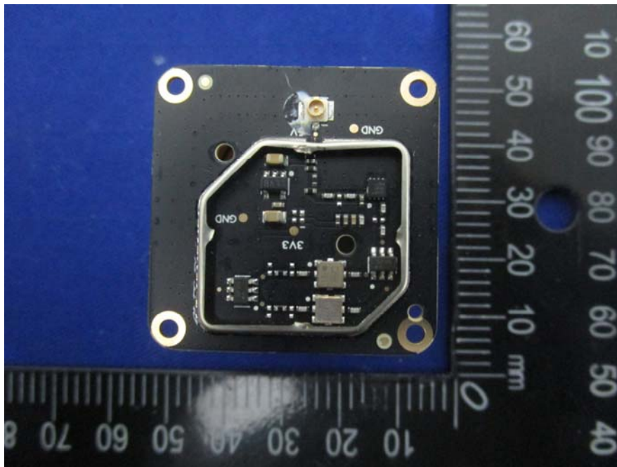
EUT – PCB-15 Bottom Uncover View
