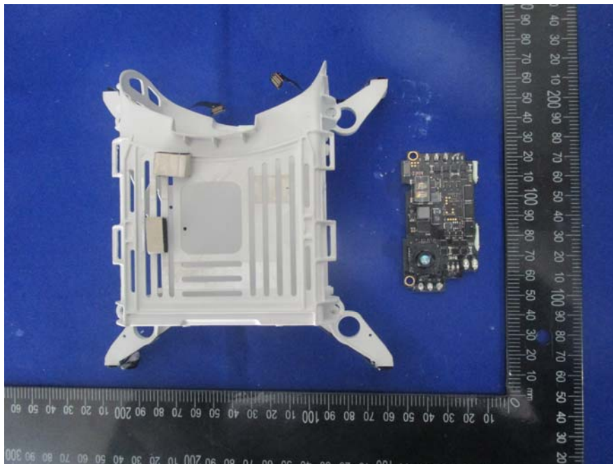
EUT –Uncover-22 View
