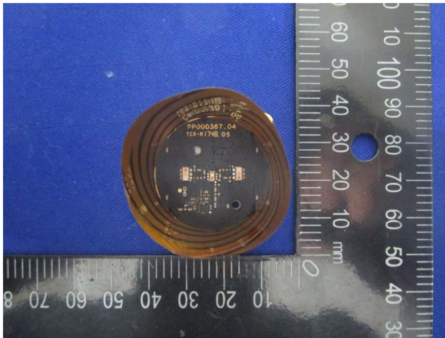
EUT – PCB-15 Top View
