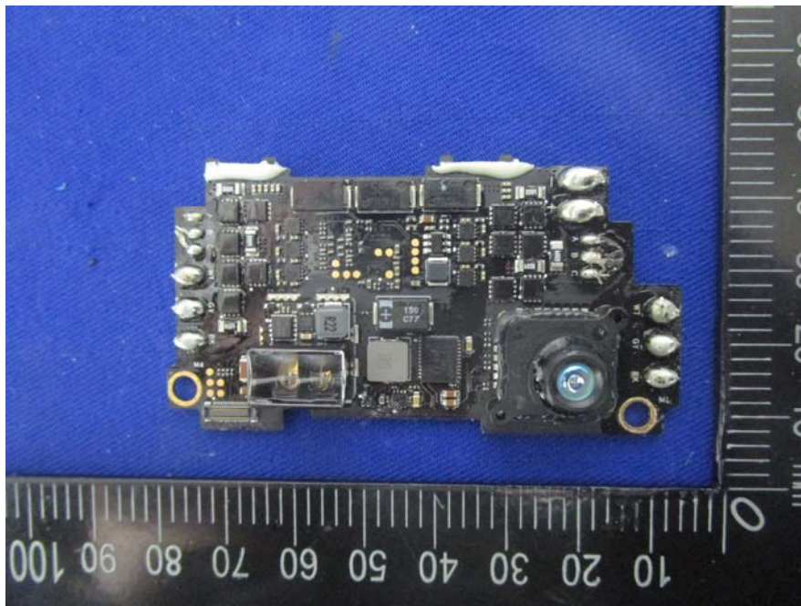
EUT – PCB-13 Top View
