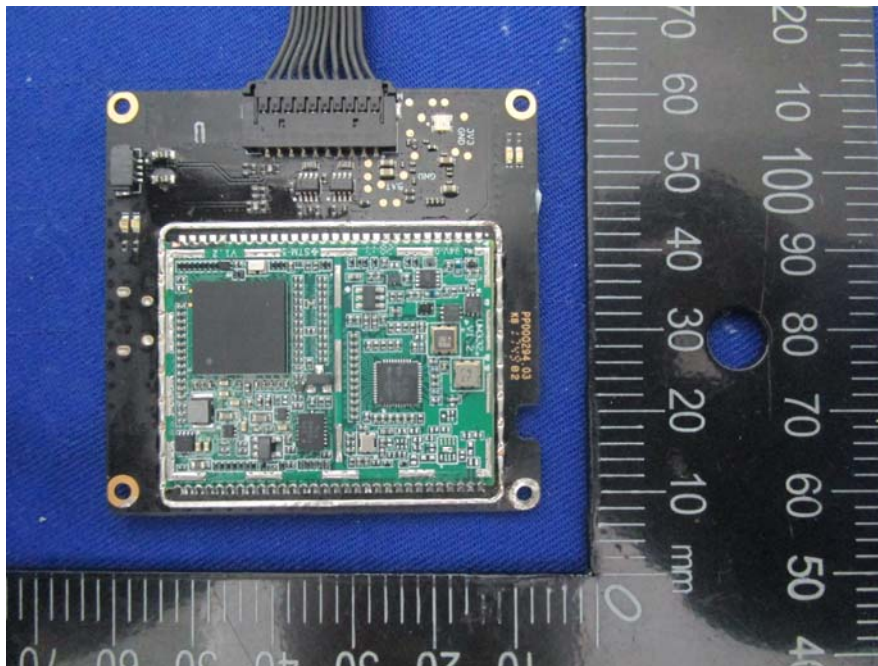
EUT – PCB-14 Top Uncover View
