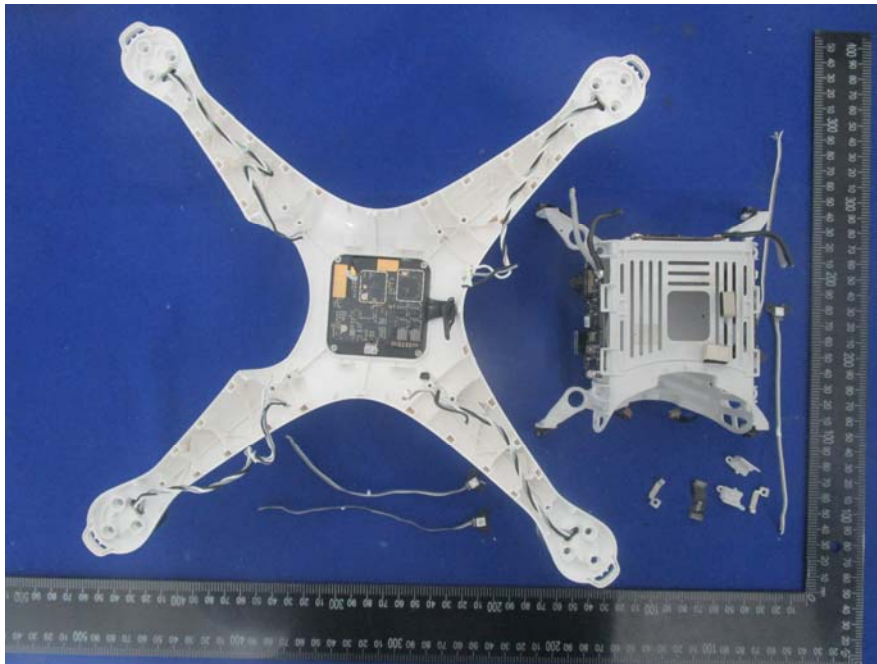
EUT – Uncover-19 View
