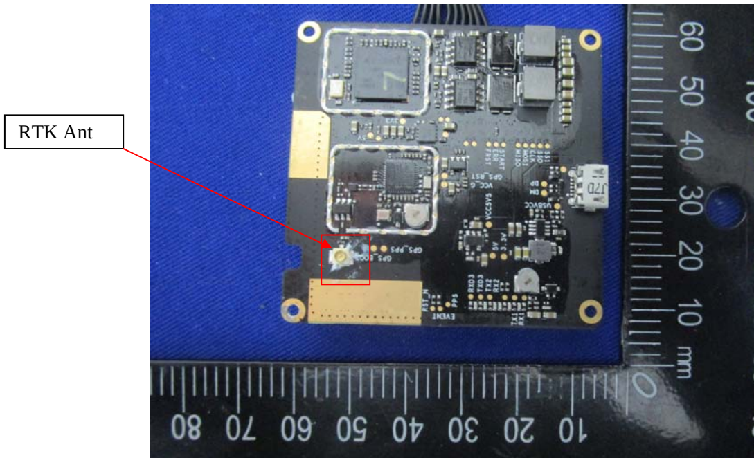
EUT – PCB-14 Bottom View
