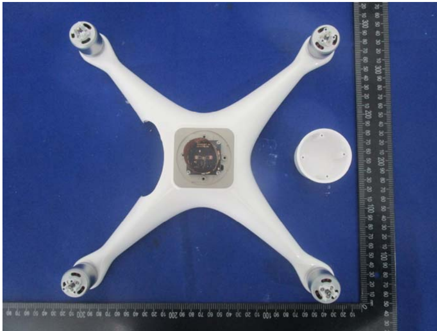
EUT – Uncover-24 View
