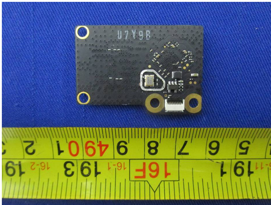
EUT – WIFI Module Bottom Uncover View
