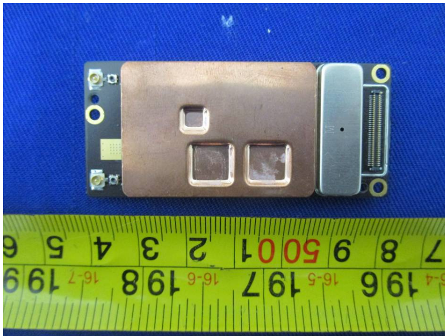
EUT – SDR Module Top View
