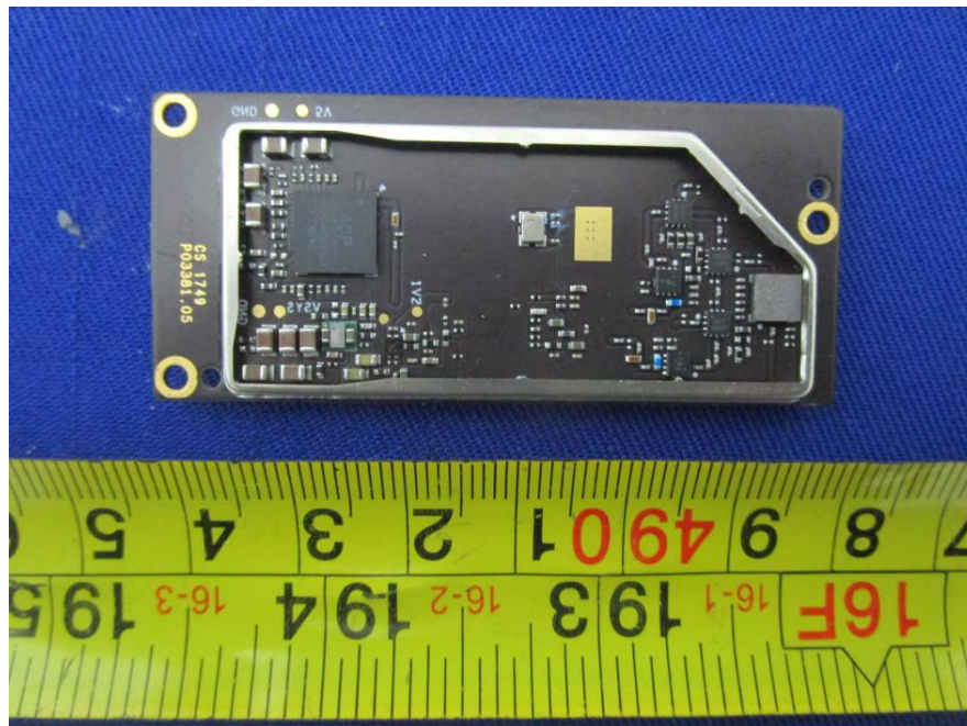
EUT – SDR Module Bottom Uncover View
