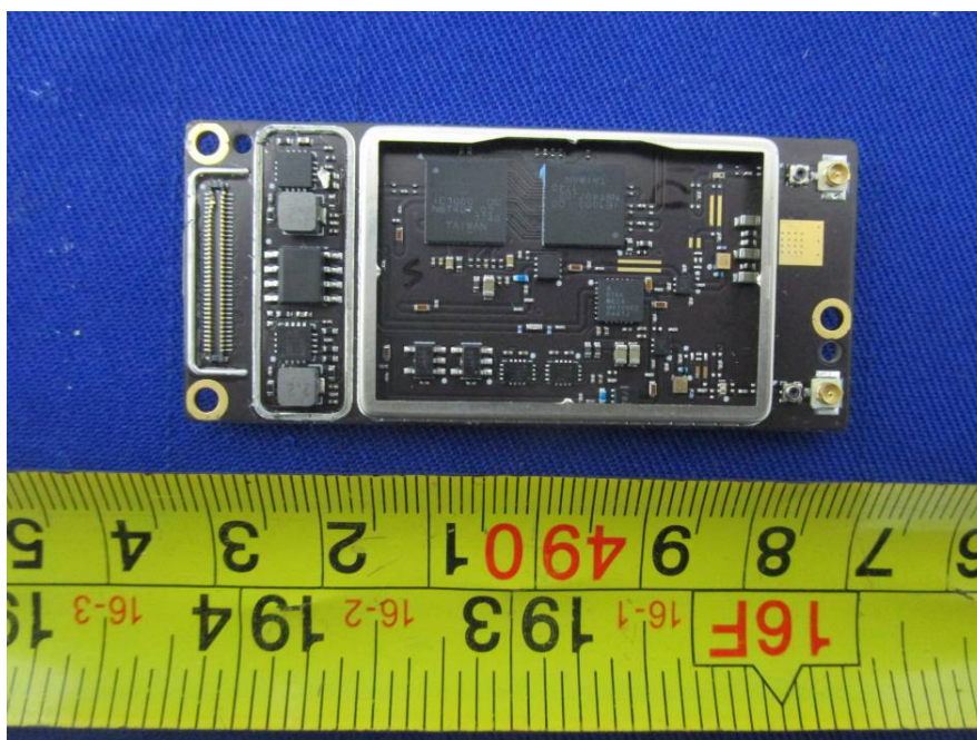
EUT – SDR Module Top Uncover View
