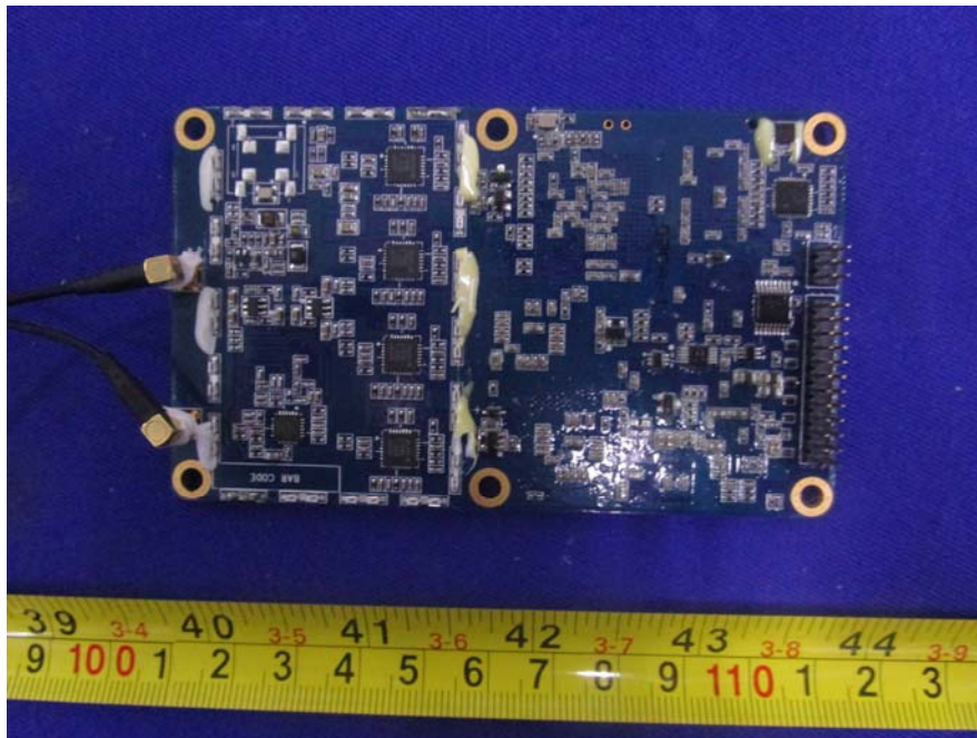
EUT- Board-3 Bottom Unshielded View
