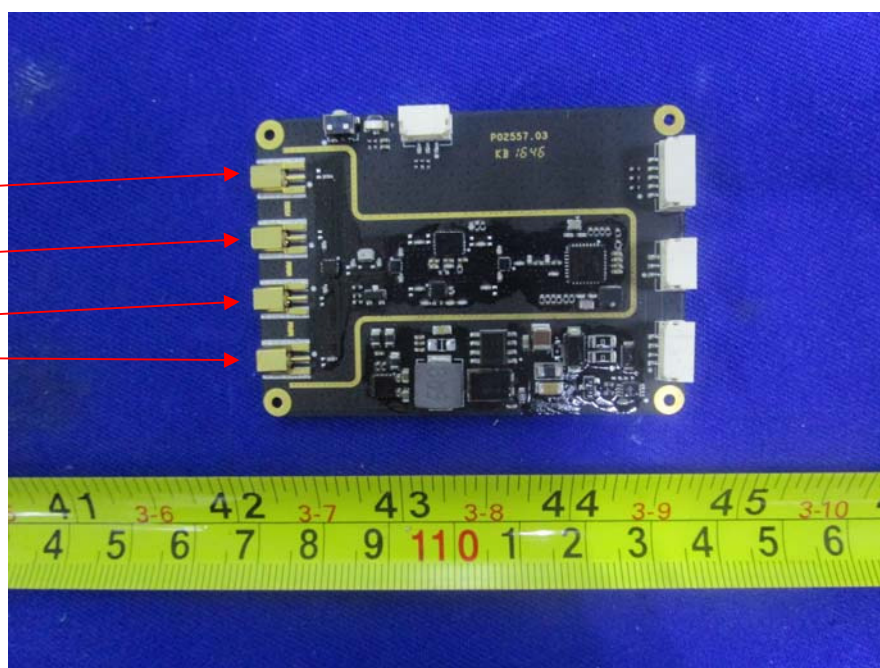
EUT- 2.4G Board Top View
