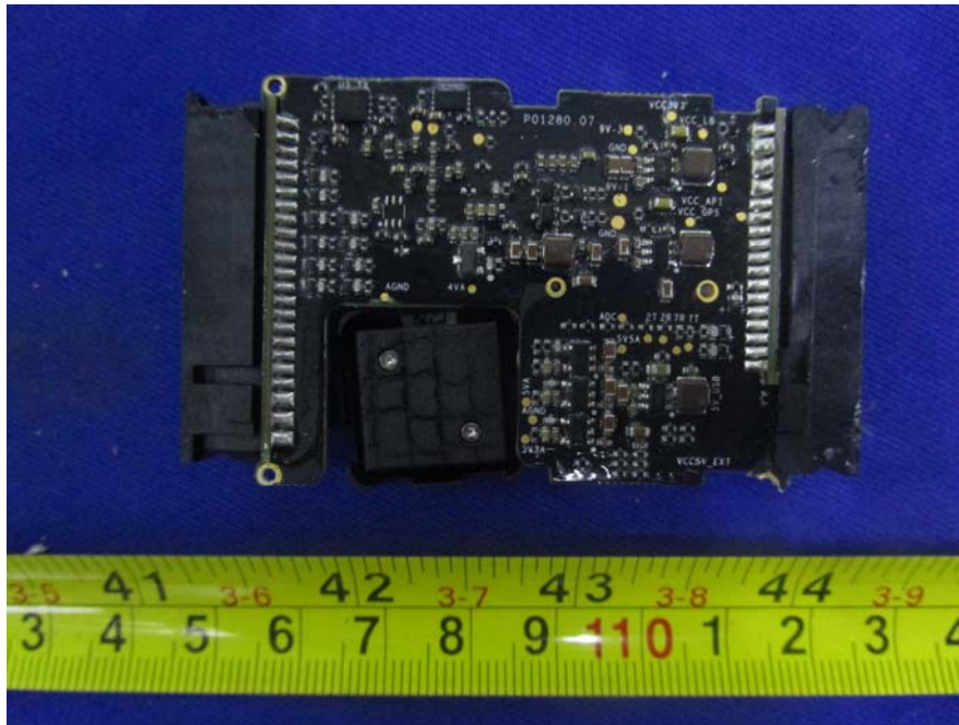
EUT- Board-4 Bottom View
