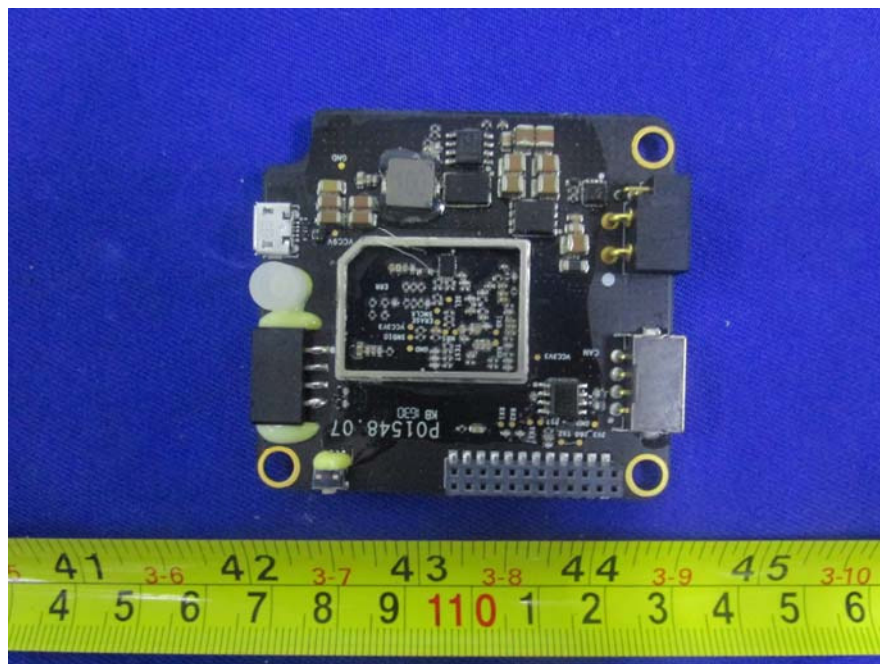
EUT- Board-2 Top Unshielded View
