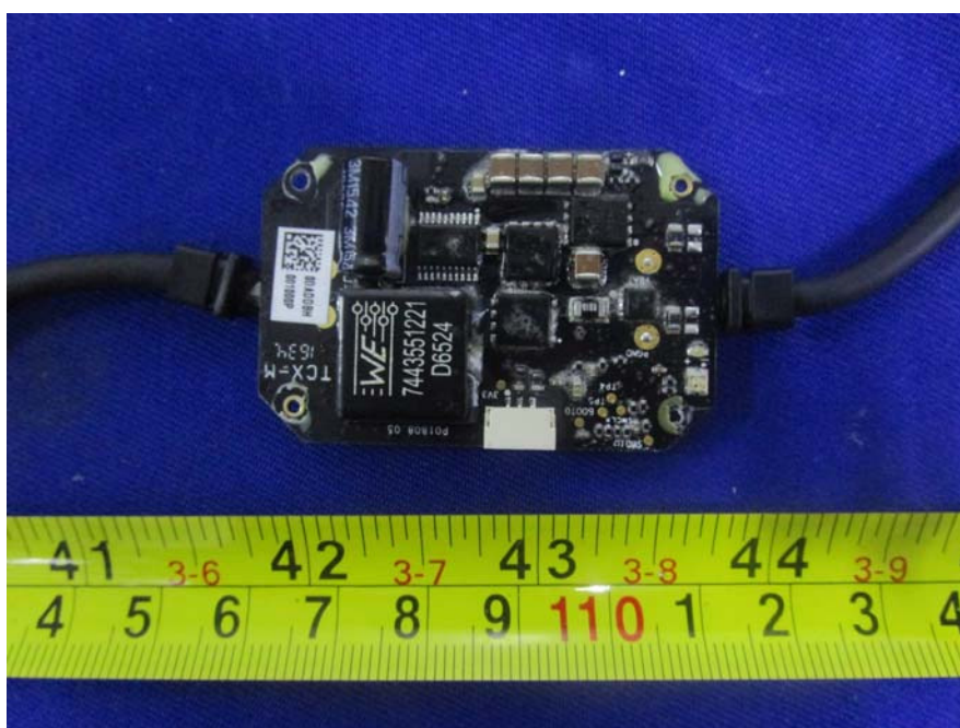
EUT- Board-6 Top View
