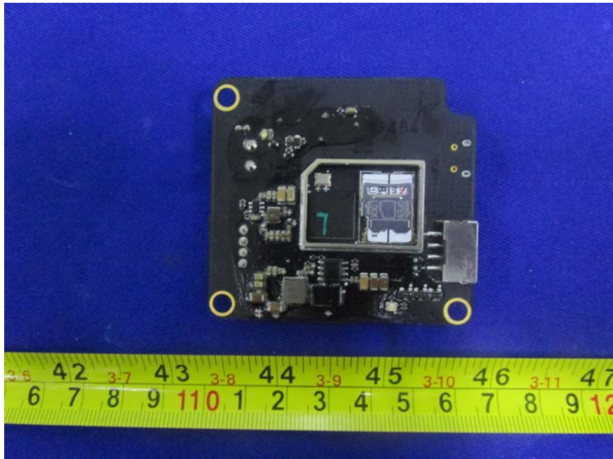
EUT- Board-2 Bottom Unshielded View
