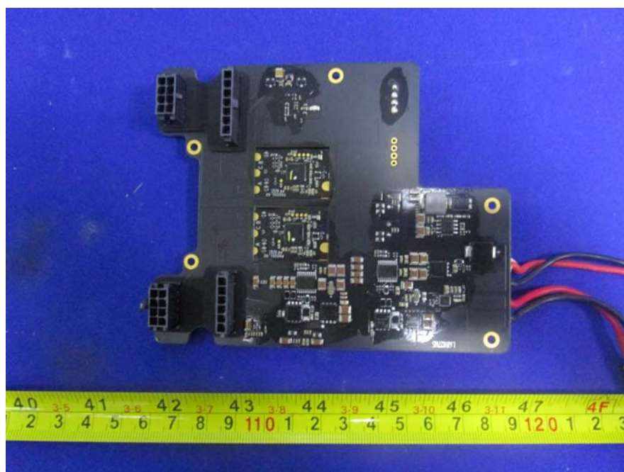
EUT- Board-7 Top View
