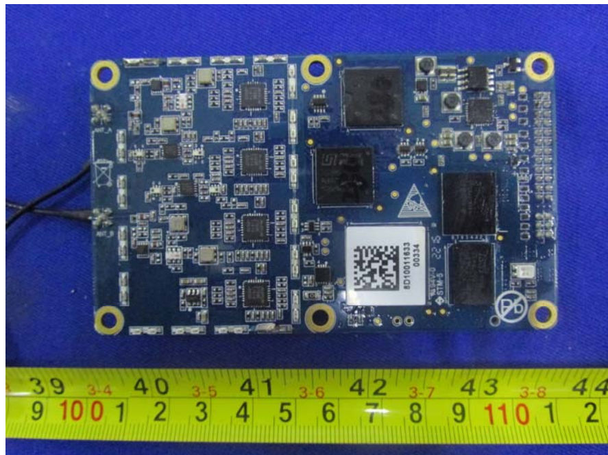
EUT- Board-3 Top Unshielded View
