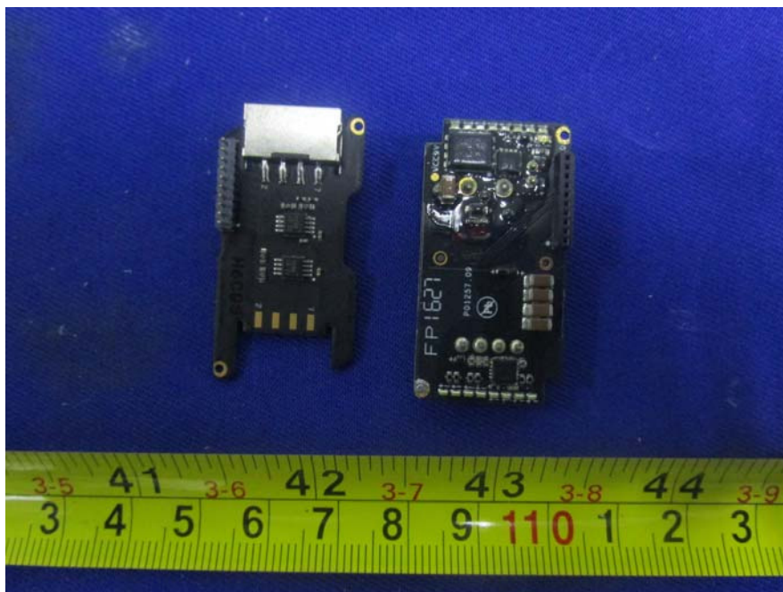
EUT- Board-5 Top View
