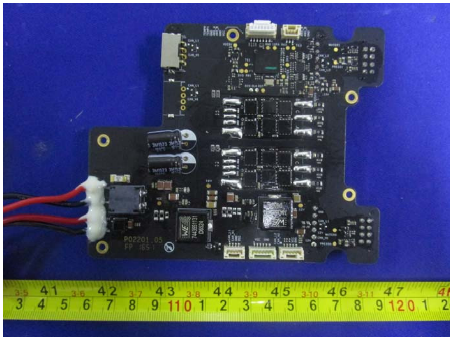
EUT- Board-7 Bottom View
