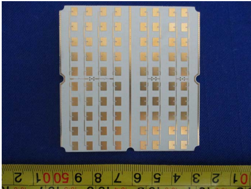
EUT –Antenna Board Top View
